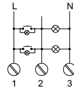
3 wires connection
