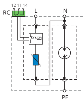
Internal configuration
