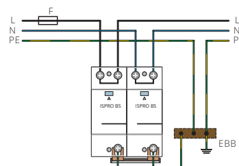
TN-S Network - Single-phase (V-connection)
