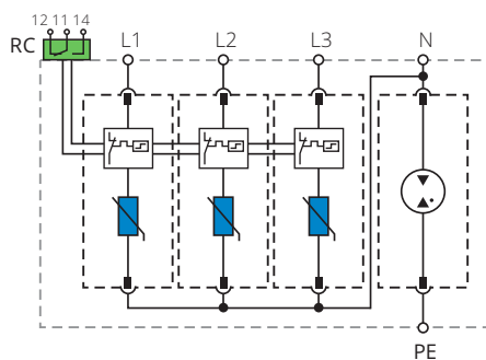
Internal configuration
