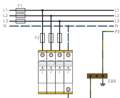
IT Network - (Three-phase)
