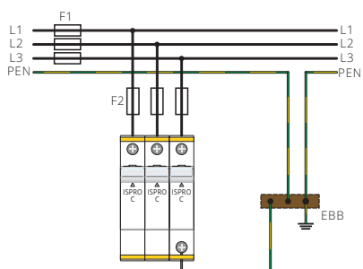
TN-C Network - (Three-phase)
