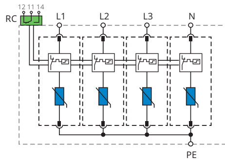
Internal configuration
