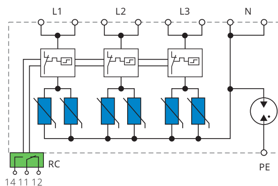
Internal configuration
