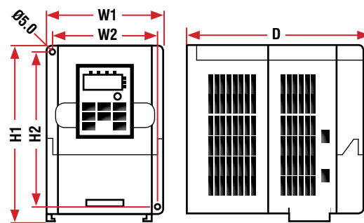
Wall mounting (unit: mm)
